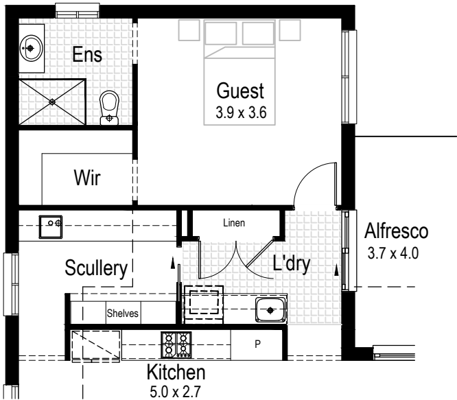
Alternative Scullery & Laundry option
